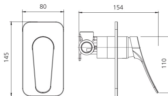
Trim kit and inwall body assembly.
