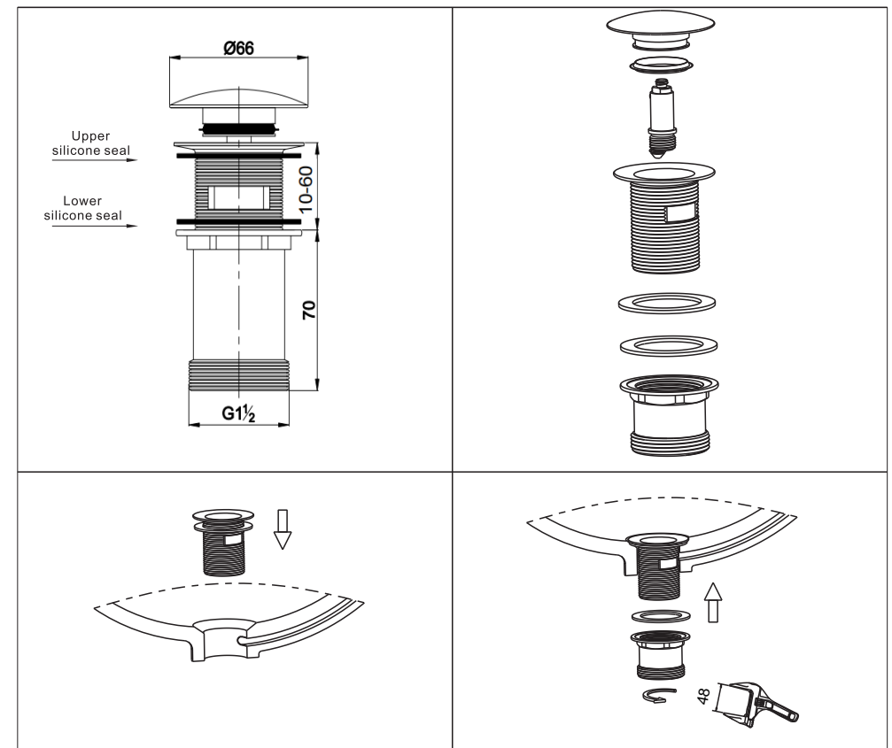
Pop-up Waste Product code: ACC706-R-GW
